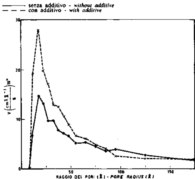
8 - Pore size distribution curves in the Portland n° 3 cement pastes hydrated 7 days with and without \text{CaCl}_2 .
