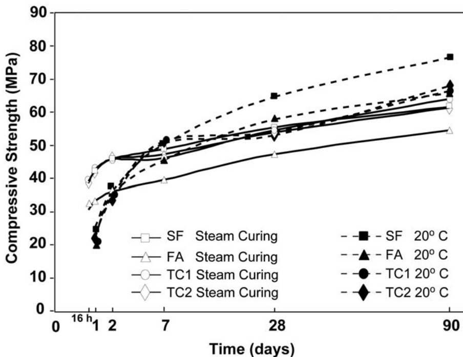
Figure 4: Compressive strength of flowing concretes.
