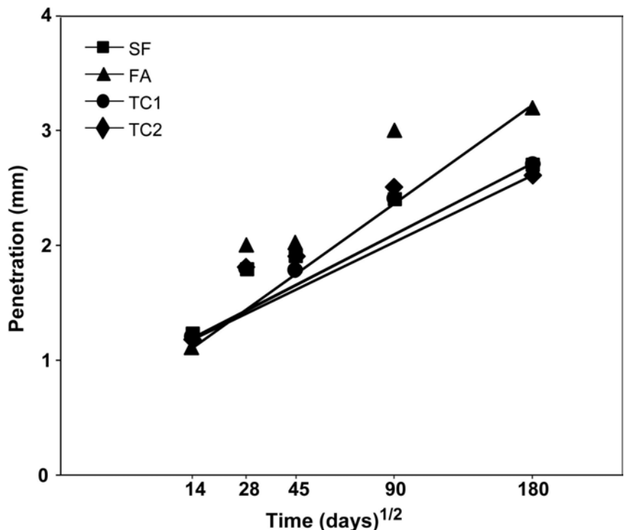
Figure 8: Penetration of Cl - in SCC cured at 20°C.
