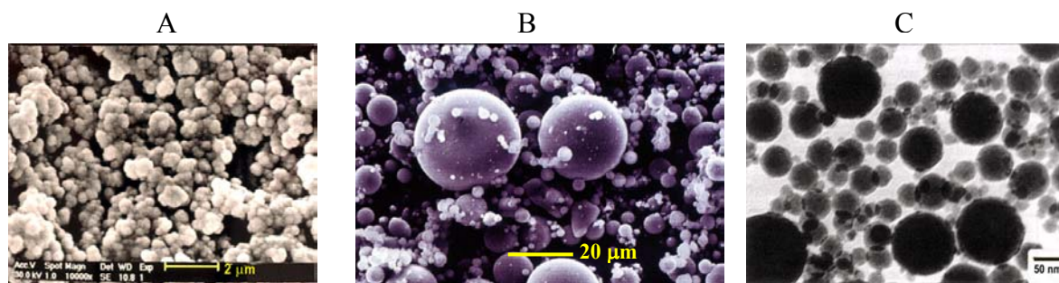
Figure 2: SEM micrographs showing: silica fume (A), fly ash (B) and UFACS (C)
