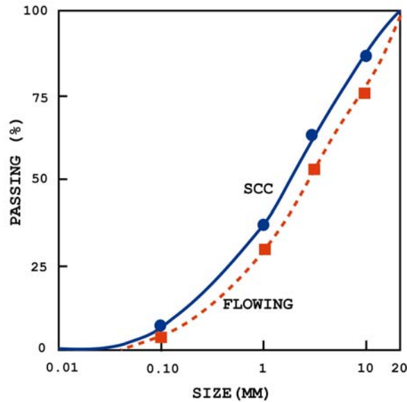
Figure 3: Particle size distribution of aggregates for flowing and self-compacting concretes.
