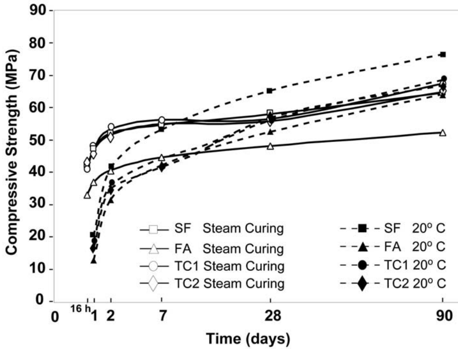
Figure 5: Compressive strength of SCC.
