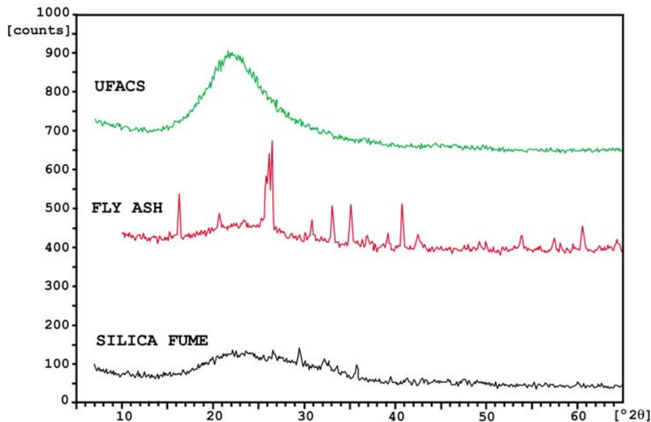
Figure 1: XRD patterns of silica fume, fly ash and UFACS.
