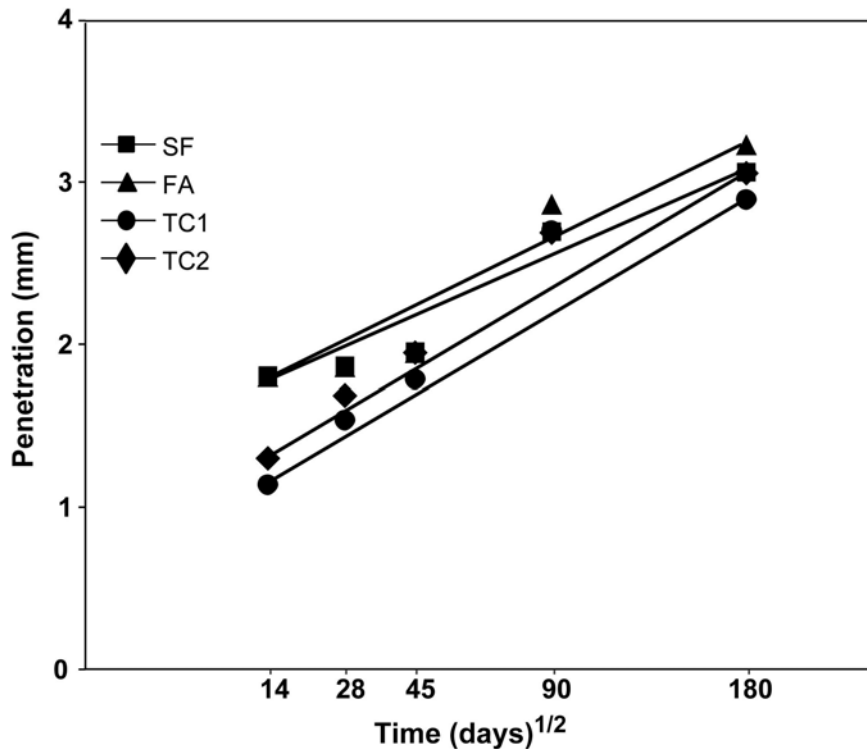
Figure 6: Penetration of Cl - in flowing concretes cured at 20°C.
