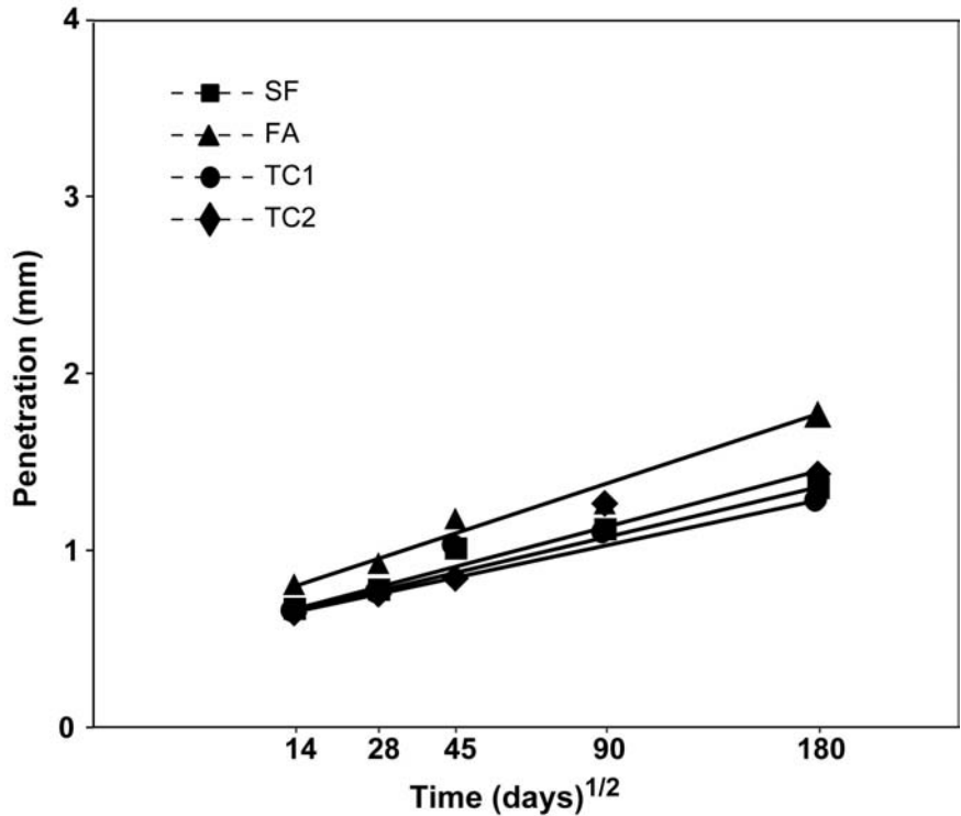
Figure 7: Penetration of CO 2 in flowing concretes cured at 20°C.
