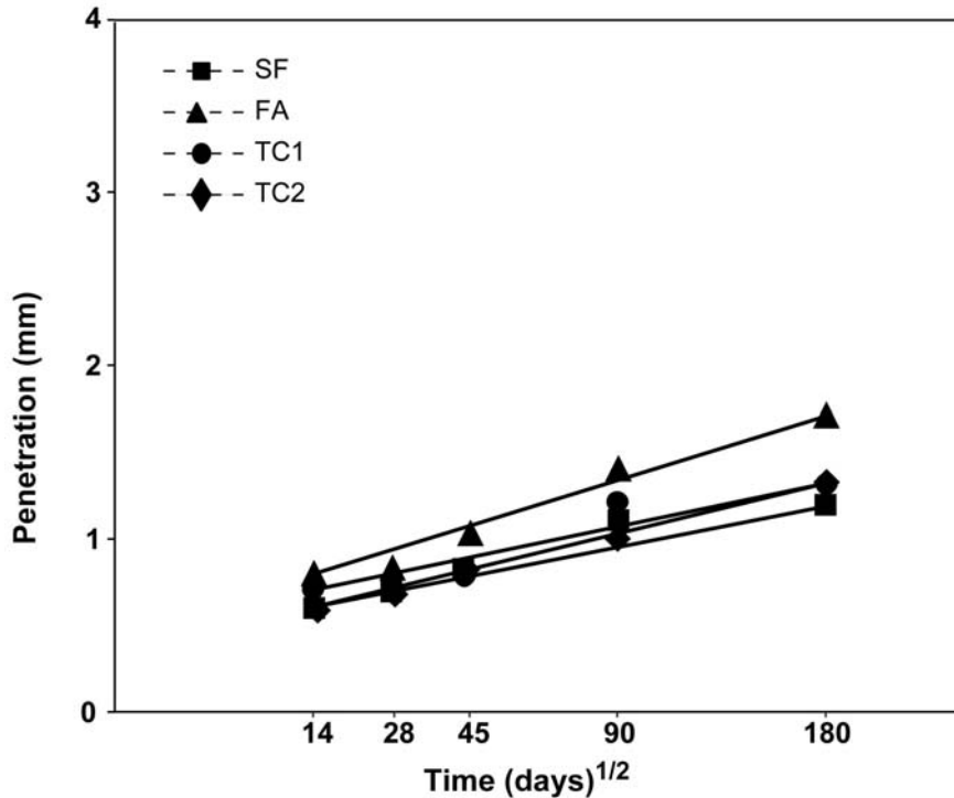
Figure 9: Penetration of CO 2 in SCC cured at 20°C.
