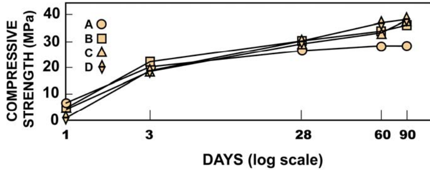
Fig. 3 – Compressive strength as a function of time of SCC with different mineral additions (Table 3).
