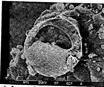
Figure 13. SEM micrograph of a cenosphere in fly ash
