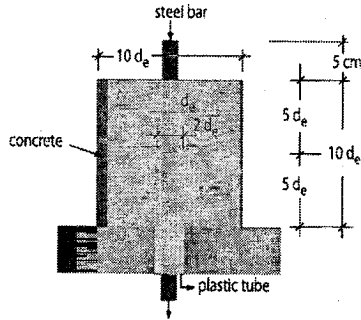
Figure 3. Reinforced specimen for the steel-concrete bond test according to RILEM-CEB
