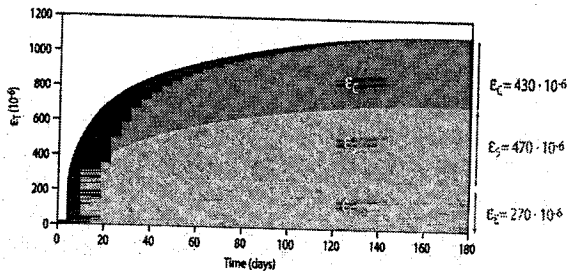
Figure 12. OFC: elastic strain ( \epsilon_E ), drying-shrinkage ( \epsilon_S ) and creep strain ( \epsilon_C ) at R.H. of 65% with a load of 163 MPa at 7 days (1/4 of 65 MPa)
