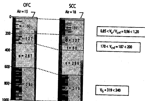
Figure 2. Composition in volume ( L/m^3 ) of the ingredients in the ordinary concrete (OC) and SCC
