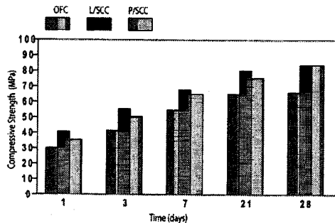
Figure 4. Compressive strength of OFC, L/SCC and F/SCC
