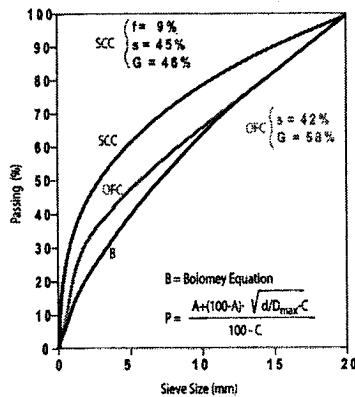
Figure 1. Particle size distribution of the aggregate in L/SCC or ordinary flowing concrete (OFC) in comparison with the Bolomey equation; f= ground limestone; s= sand; G = gravel
