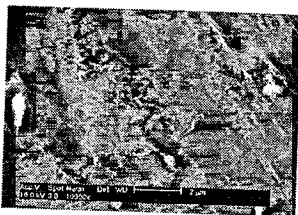
Figure 5. SEM micrograph of the cement matrix of OFC (by D. Salvioni, Mapei)
