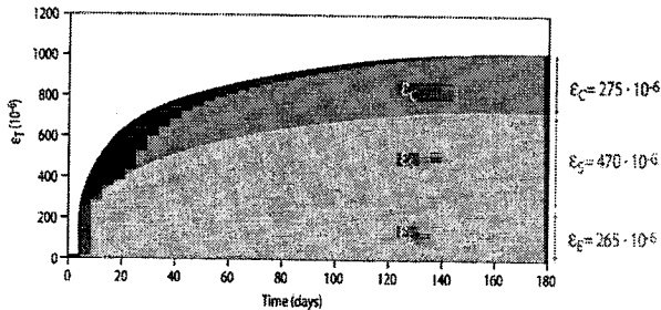
Figure 10. OFC: elastic strain ( \epsilon_E ), drying-shrinkage ( \epsilon_S ) and creep strain ( \epsilon_C ) at R.H. of 65% with a load of 138 MPa at 7 days (1/4 of 55 MPa)
