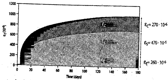
Figure 11. OFC: elastic strain ( \epsilon_E ), drying-shrinkage ( \epsilon_S ) and creep strain ( \epsilon_C ) at R.H. of 65% with a load of 170 MPa at 7 days (1/4 of 68 MPa)
