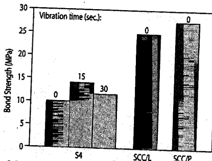
Figure 8. Steel bond-strength of OFC and SCCs. The figures indicate the vibration time.
