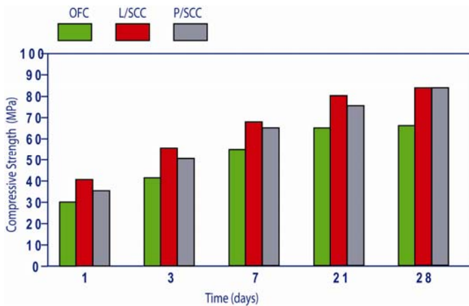
Figure 4. Compressive Strength of OFC, L/SCC and F/SCC.
