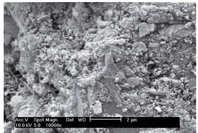
Figure 6. SEM micrograph of the cement matrix of L/SCC (by D. Salvioni, Mapei).
