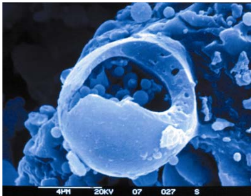
Figure 13. SEM micrograph of a cenosphere in fly ash.
