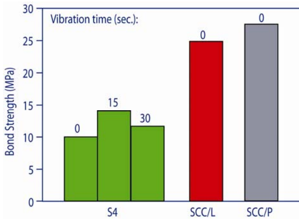
Figure 8. Steel bond-strength of OFC and SCCs. The figures indicate the vibration time.
