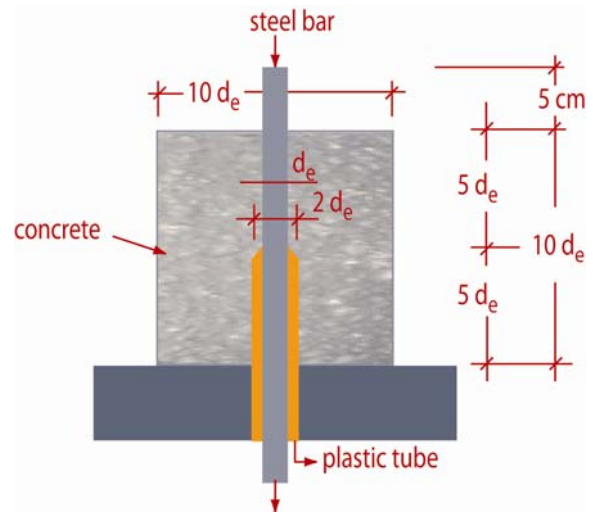
Figure 3. Reinforced specimen for the steel-concrete bond test according to RILEM-CEB.
