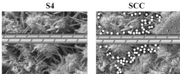
Figure 9. Schematic model of strength-concrete area in ordinary flowing concrete and in SCC.
