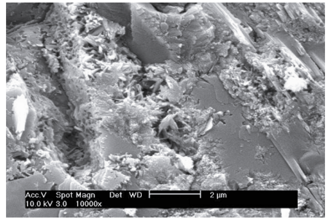
Figure 5. SEM micrograph of the cement matrix of OFC (by D. Salvioni, Mapei).
