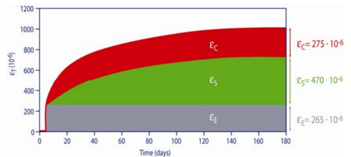
Figure 10. OFC: elastic strain ( \epsilon_E ), drying-shrinkage ( \epsilon_S ) and creep strain ( \epsilon_C ) at R.H. of 65% with a load of 13.8 MPa at 7 days (1/4 of 55 MPa).
